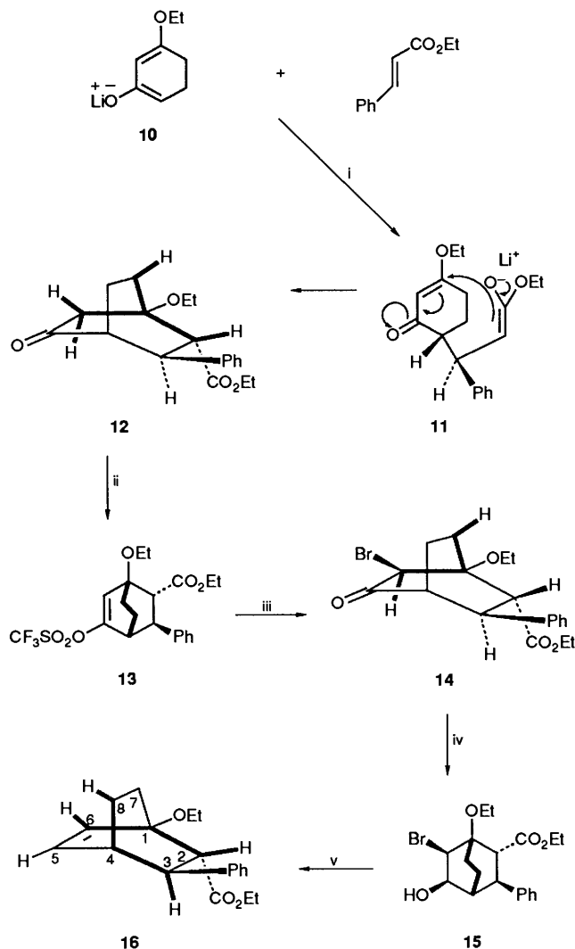
Scheme 4 Reagents: i, THF, -70^{\circ}\text{C} , 1 h; NH 4 Cl(aq), 75%; ii, Et 3 N, TMSOTf, 0^{\circ}\text{C} \rightarrow room temp., 1.5 h; iii, NBS, CH 2 Cl 2 , 5 min, 86%; iv, NaBH 4 , THF-EtOH-H 2 O, 82%; v Zn (act.), EtOH, heat, 1 h, 99%
